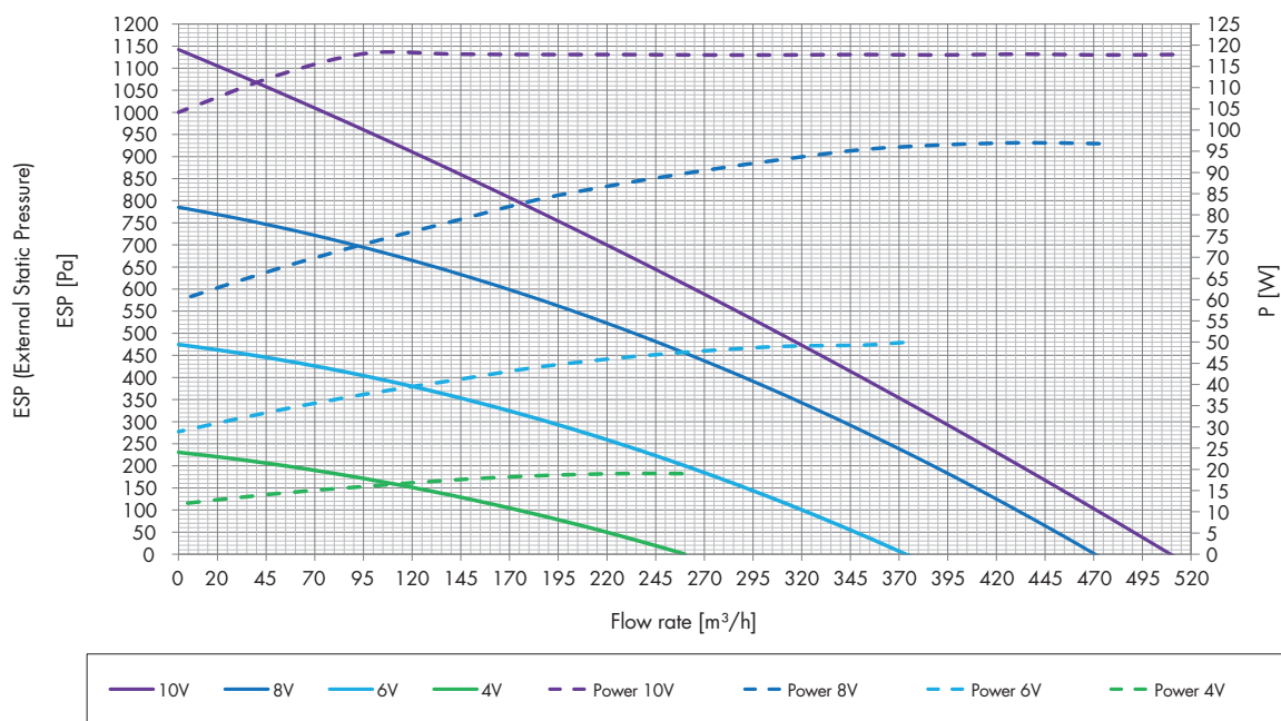
Fan curves for the Endura Delta 450 pressure based on flow rate
